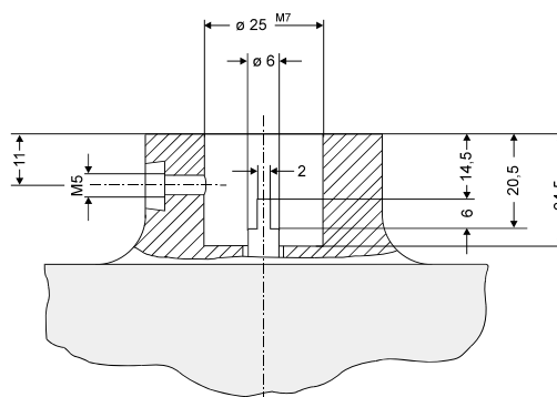
Dimensions of the drive shaft coupling
