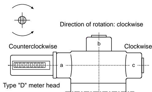
Direction of rotation of the drive shafts
