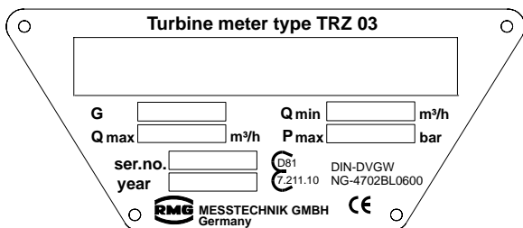
Main data plate of the TRZ 03 turbine meter with type “F” meter head
